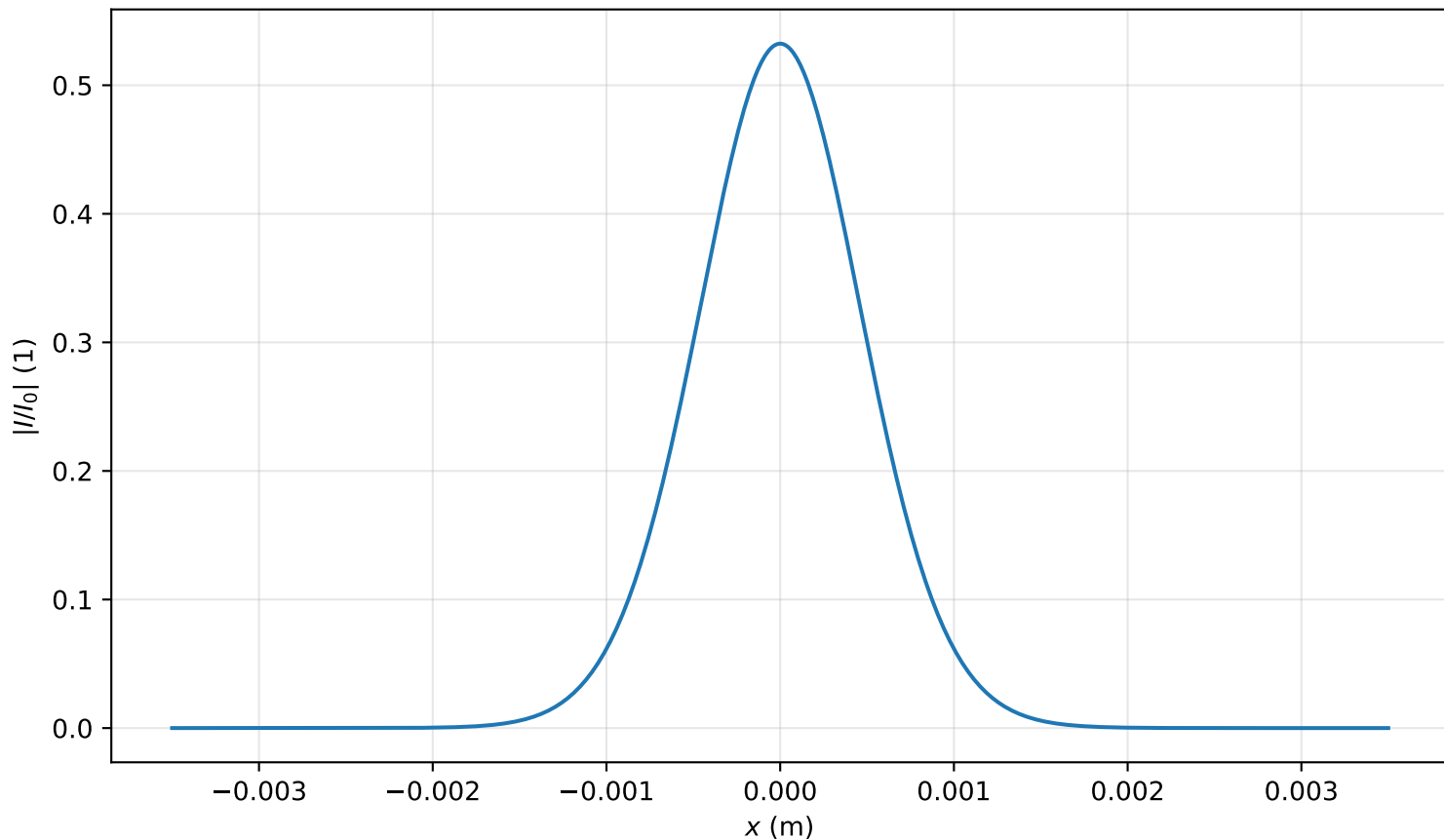
Intensity profile I(x, y = 0, z = 2.229m)/I_0 , P_{in}=0.2P_{cr} , artificial time
